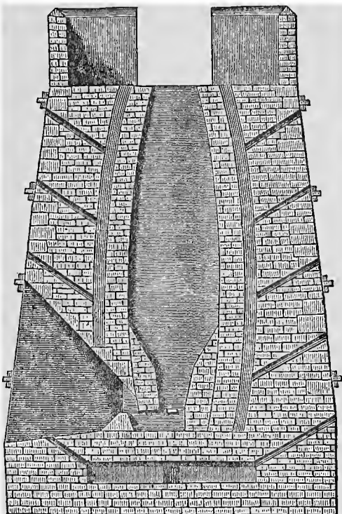
FIG. 8. A NORWEGIAN BLOOMERY FURNACE (Eighteenth century)
